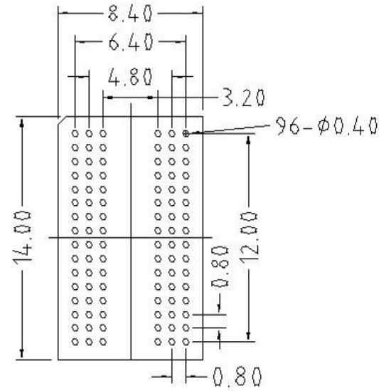
PCB PATTERN (Top View)
