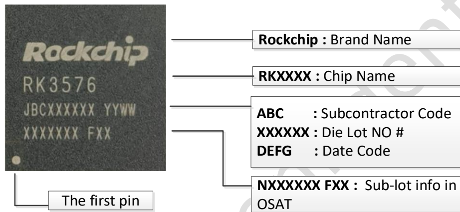
Fig.2-1 Package Definition
